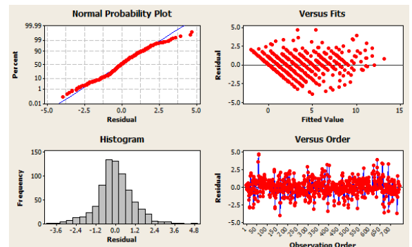
Figure 2: Residual plot of initial full model
