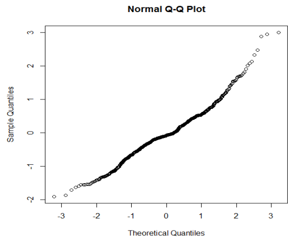
Figure 8. Normal probability plot of the transformed model
