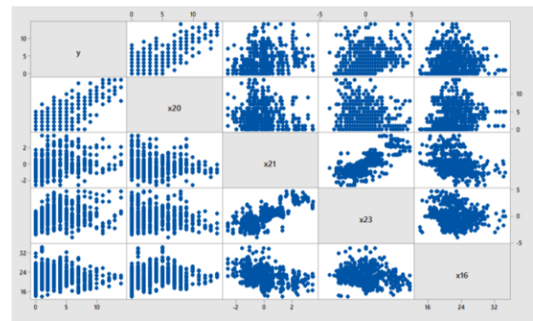
Figure 1: Scatter plot for the initial model
