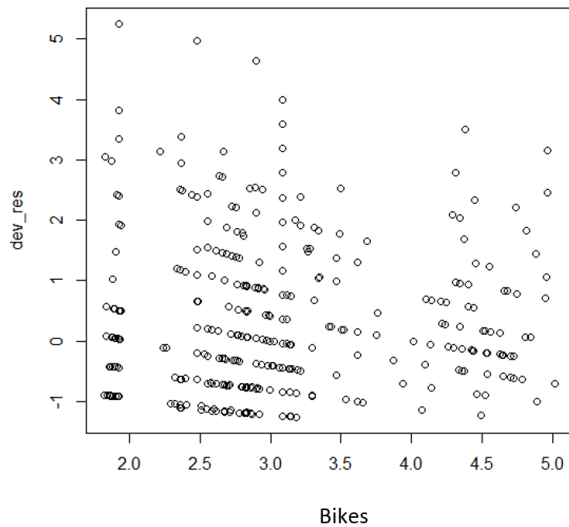
Figure 9. Deviance Residual plot of the transformed model
