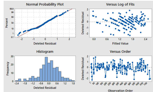
Figure 6. Residual plot after transformation
