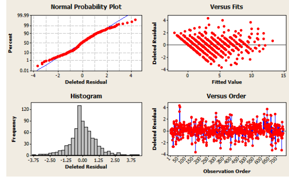
Figure 3: Residual plot of subset regression
