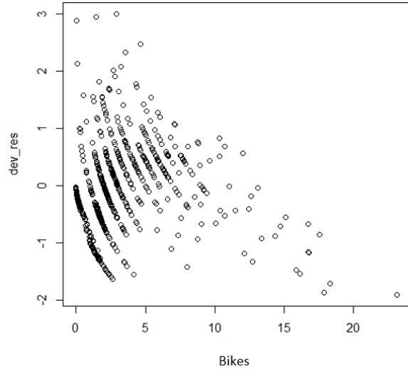
Figure 7. Deviance Residual plot of initial model
