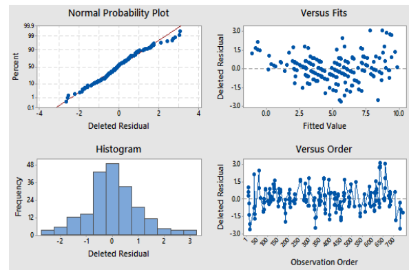
Figure 4: Residual plot of final model
