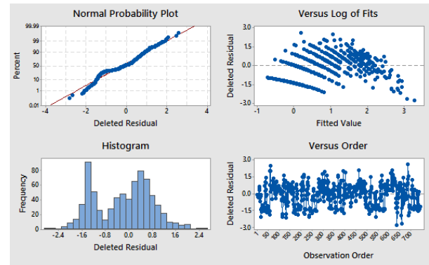
Figure 5. Residual plot for initial model of Poisson Regression
